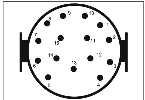
Fig. 12-5: Presa ISO12098, 15 poli
