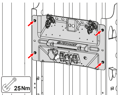
Koblingsholder
